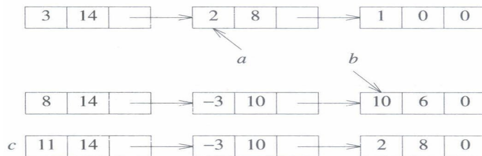
Figure: Generating the first three terms of c = a + b
