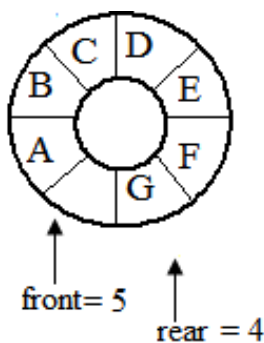
(a) A full circular queue
